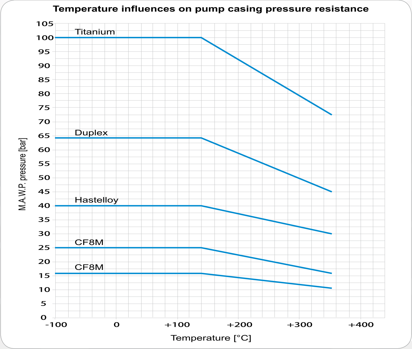
MAWP for M PUMPS CN MAG-M series ISO 2858 - DIN 24256
